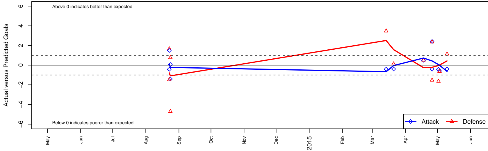
Breakers Red G99 Dots are actual minus expected GF (blue circles) and GA (red triangles). Blue line is smoothed change in attack strength. Red is smoothed change in defense strength.
